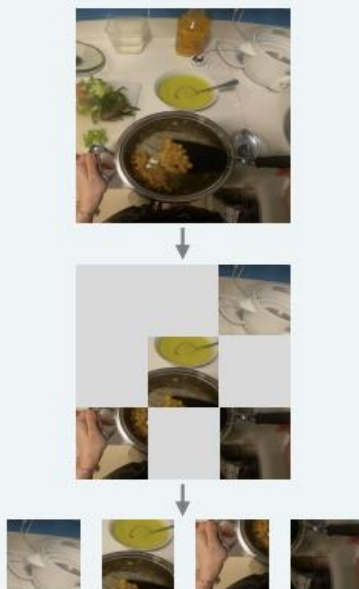
(a) Masking
