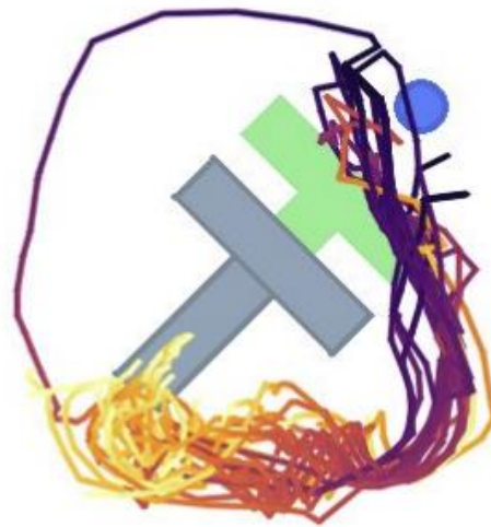
LSTM-GMM
